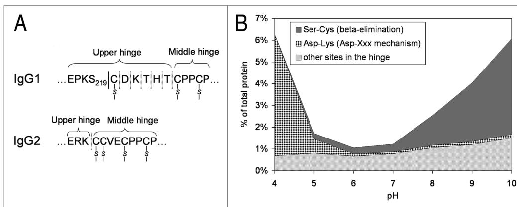
Figure 4. (A) Schematic drawing of a portion of IgG1 and IgG2 hinge region indicating sites of fragmentation. (B) pH-dependence of IgG1 hinge fragmentation monitored by SEC. Fragmentation between S 219 and C 220 in IgG1 that proceeds via \beta -elimination is shown as a solid line. The rest of the cleavages are shown as dotted lines. Disulfide bridges are indicated. The samples in (B) were incubated for approximately two weeks at 45°C. To identify the cleavage sites, the Fab fragments were purified by SEC and then analyzed by LC/MS. Considering the relatively wide pH range of 4–10, the cleavage sites can be divided into three groups. (1) Ser-Cys bond, where cleavage occurs via beta elimination, becomes dominant at higher pH. (2) Asp-Lys bond, where cleavage dramatically increases at pH < 5, presumably involving Asp side chain. (3) The rest of the cleavage sites in the hinge, where pH dependence is not as remarkable.
